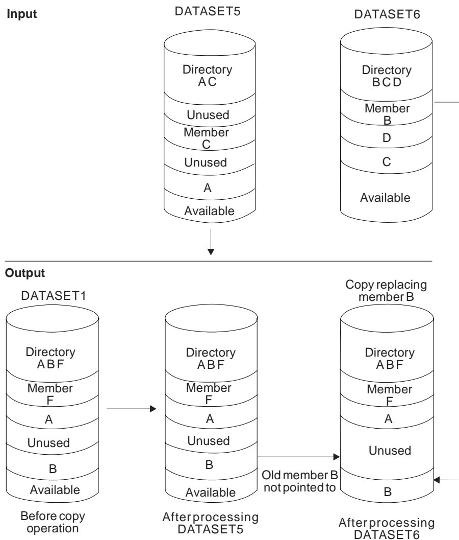
Figure 19. Selective Copy with Replace specified on the Member Level
