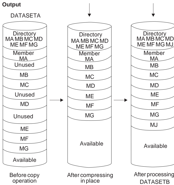
Figure 21 (Part 1 of 2). Multiple Copy Operations/Copy Steps
