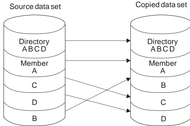
Figure 100. Partitioned Data Set Before and After an IEHMOVE Copy Operation
