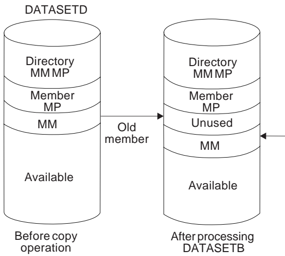
Figure 22 (Part 3 of 3). Multiple Copy Operations/Copy Steps within a Job Step
