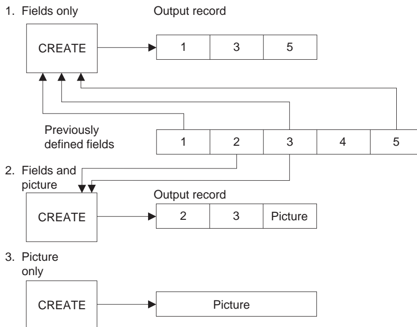
Figure 35. Creating Output Records with Utility Control Statements
