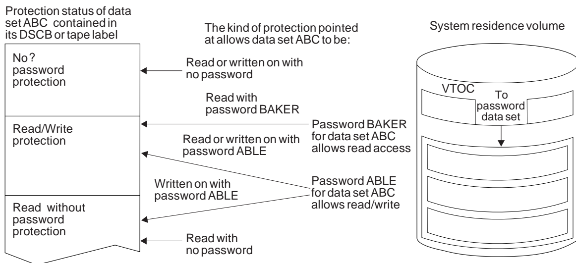
Figure 114. Relationship between the Protection Status of a Data Set and Its Passwords
