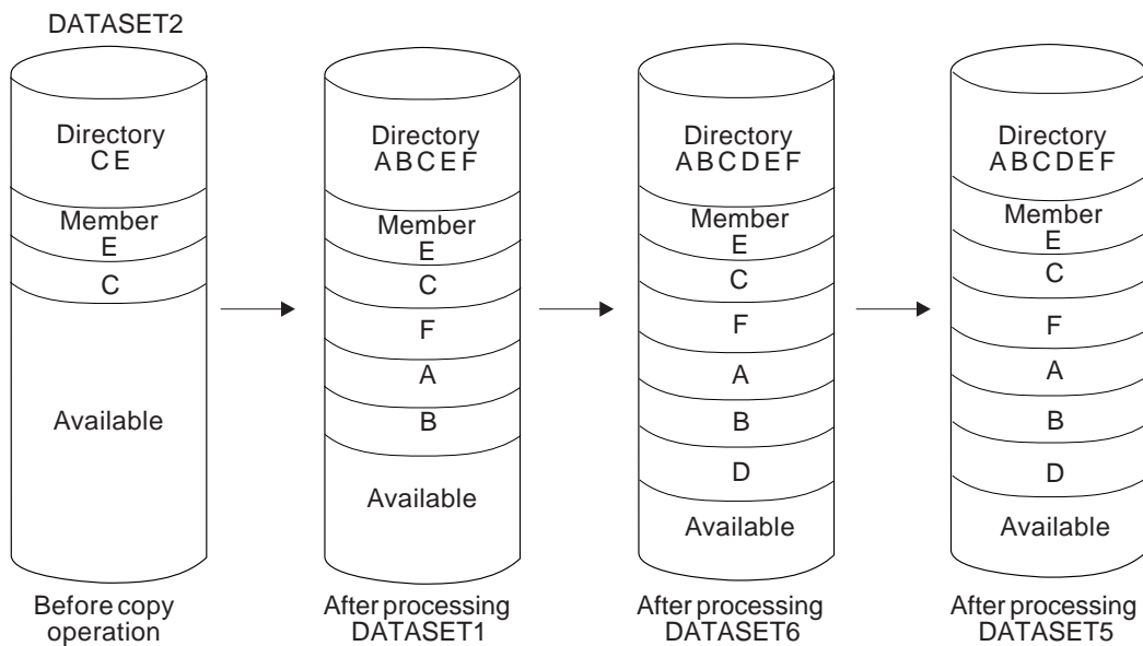
Figure 18. Copying from Three Input Partitioned Data Sets
