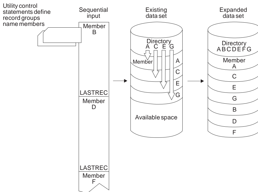
Figure 46. Adding Members to a Partitioned Data Set or PDSE Using IEBGENER
