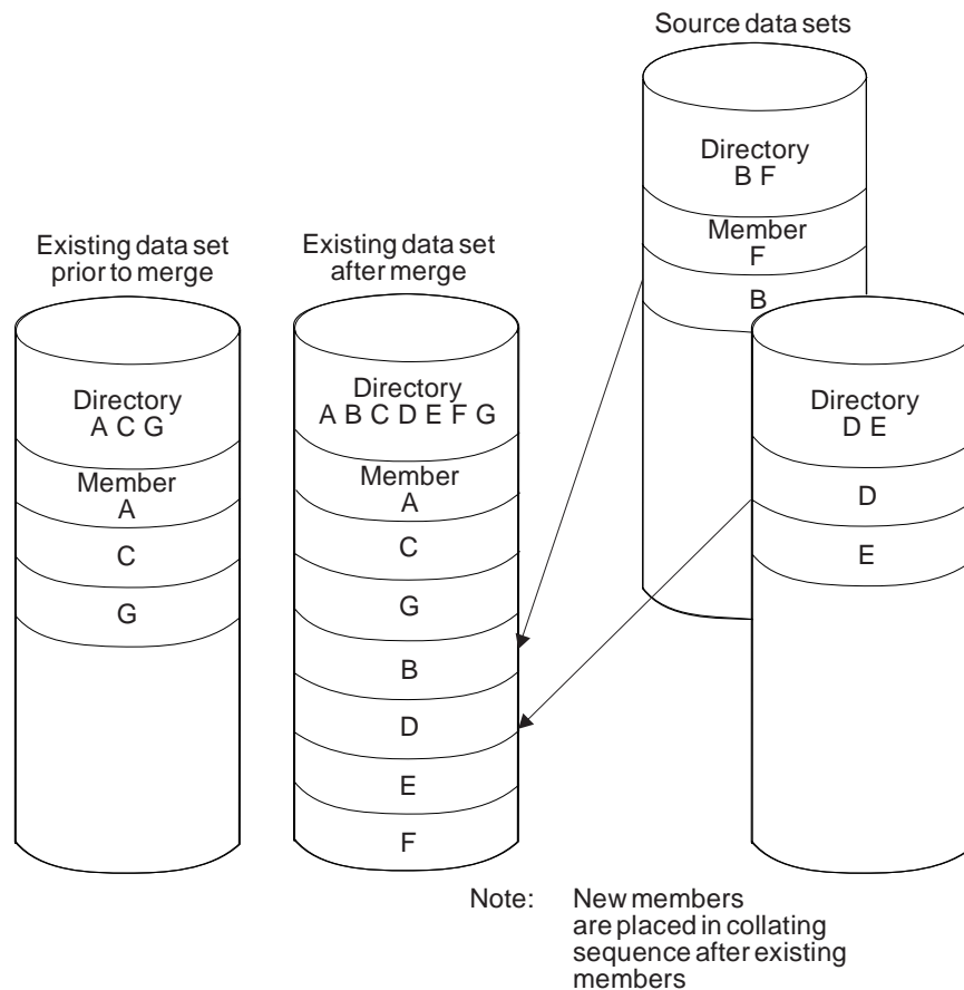
Figure 102. Merging Three Data Sets Using IEHMOVE
