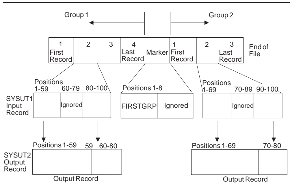
Figure 51. How a Sequential Data Set is Edited and Copied
