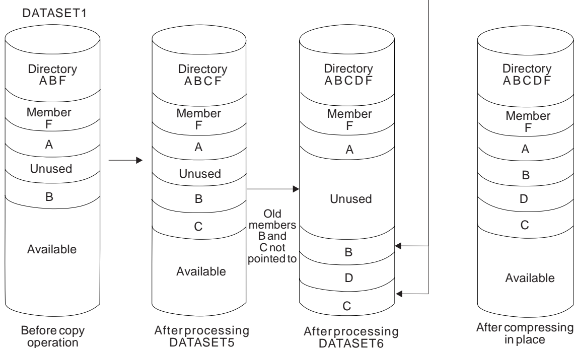
Figure 20. Compress-in-Place Following Full Copy with "Replace" Specified
