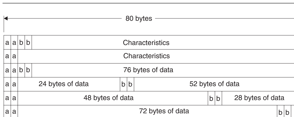
Figure 71. An Unloaded Data Set Created Using IEBISAM
