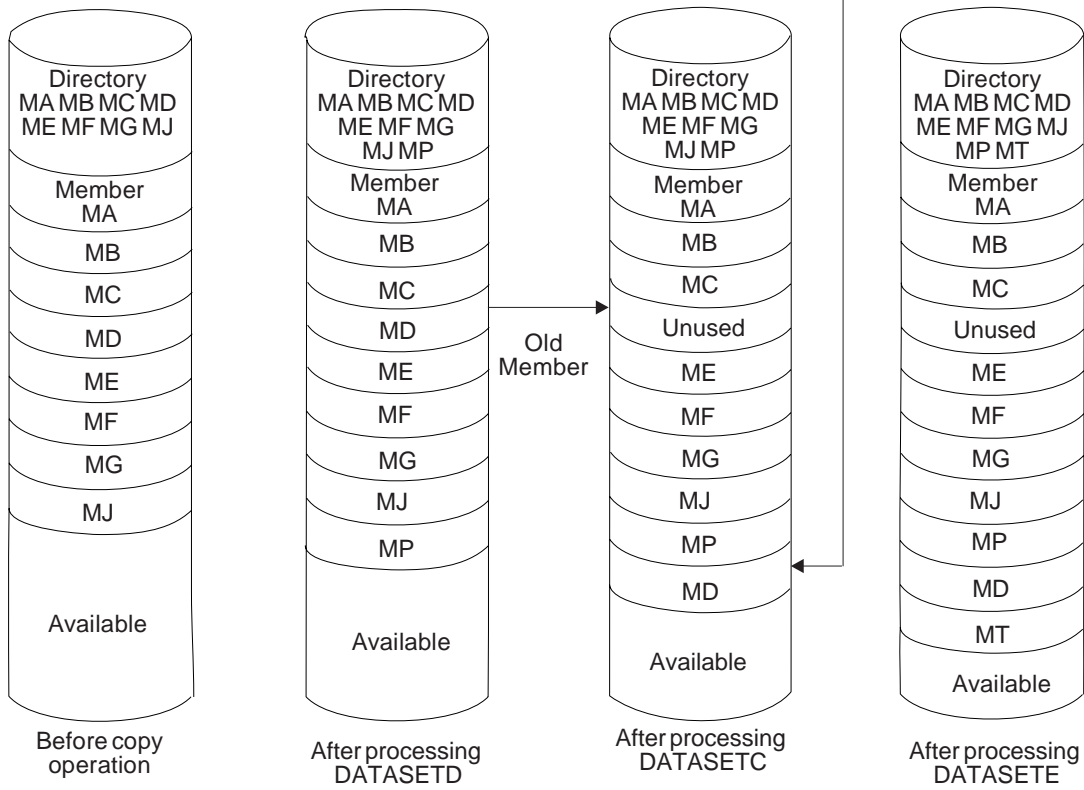
Figure 21 (Part 2 of 2). Multiple Copy Operations/Copy Steps
