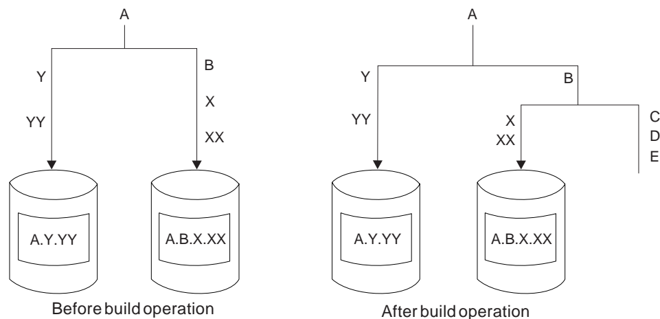
Figure 109. Index Structure Before and After an IEHPROGM Build Operation
