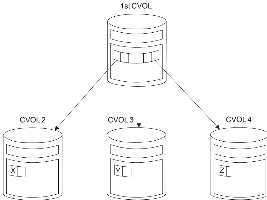
Figure 112. Connecting Three CVOLs Using IEHPROGM
