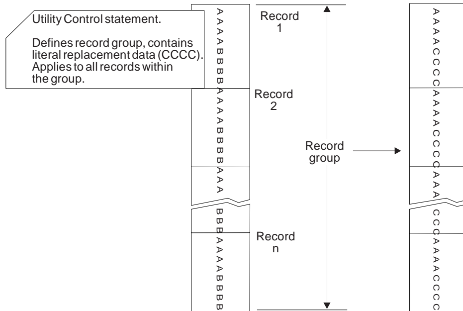
Figure 47. Editing a Sequential Data Set Using IEBGENER
