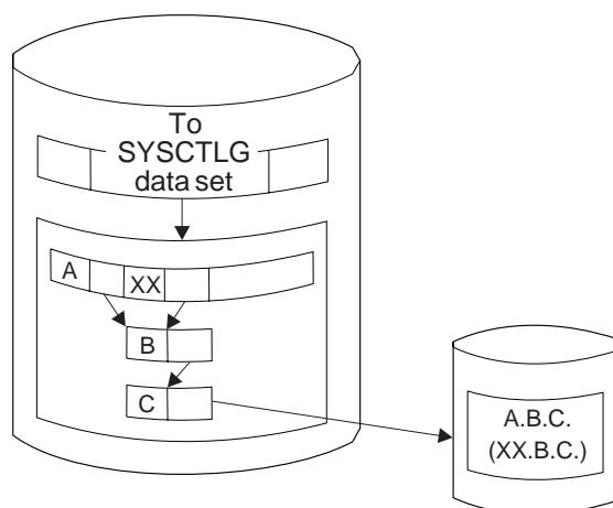
Figure 110. Building an Index Alias Using IEHPROGM
