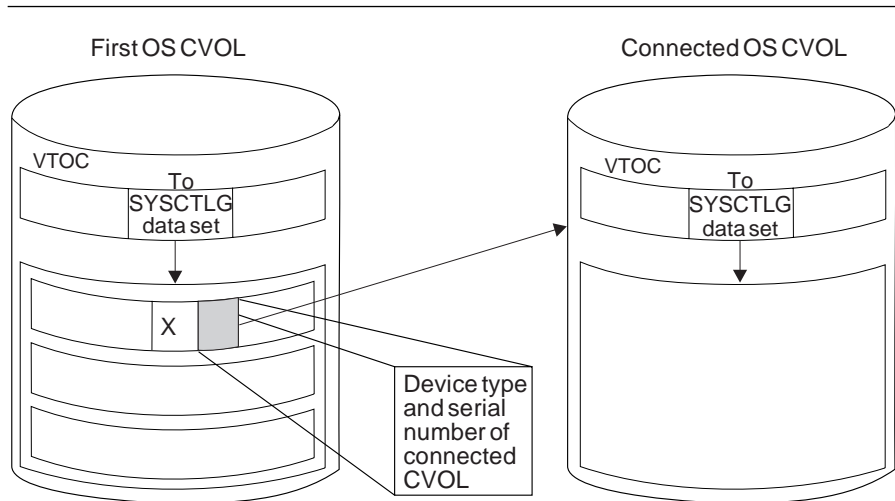
Figure 111. Connecting a CVOL to a Second CVOL Using IEHPROGM
