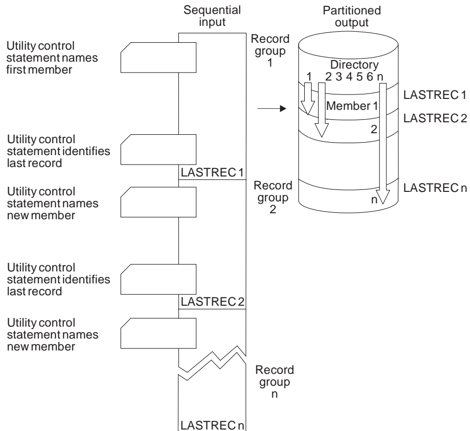
Figure 45. Creating a Partitioned Data Set or PDSE from Sequential Input Using IEBGENER
