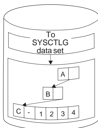
Figure 113. Building a Generation Data Group Index Using IEHPROGM
