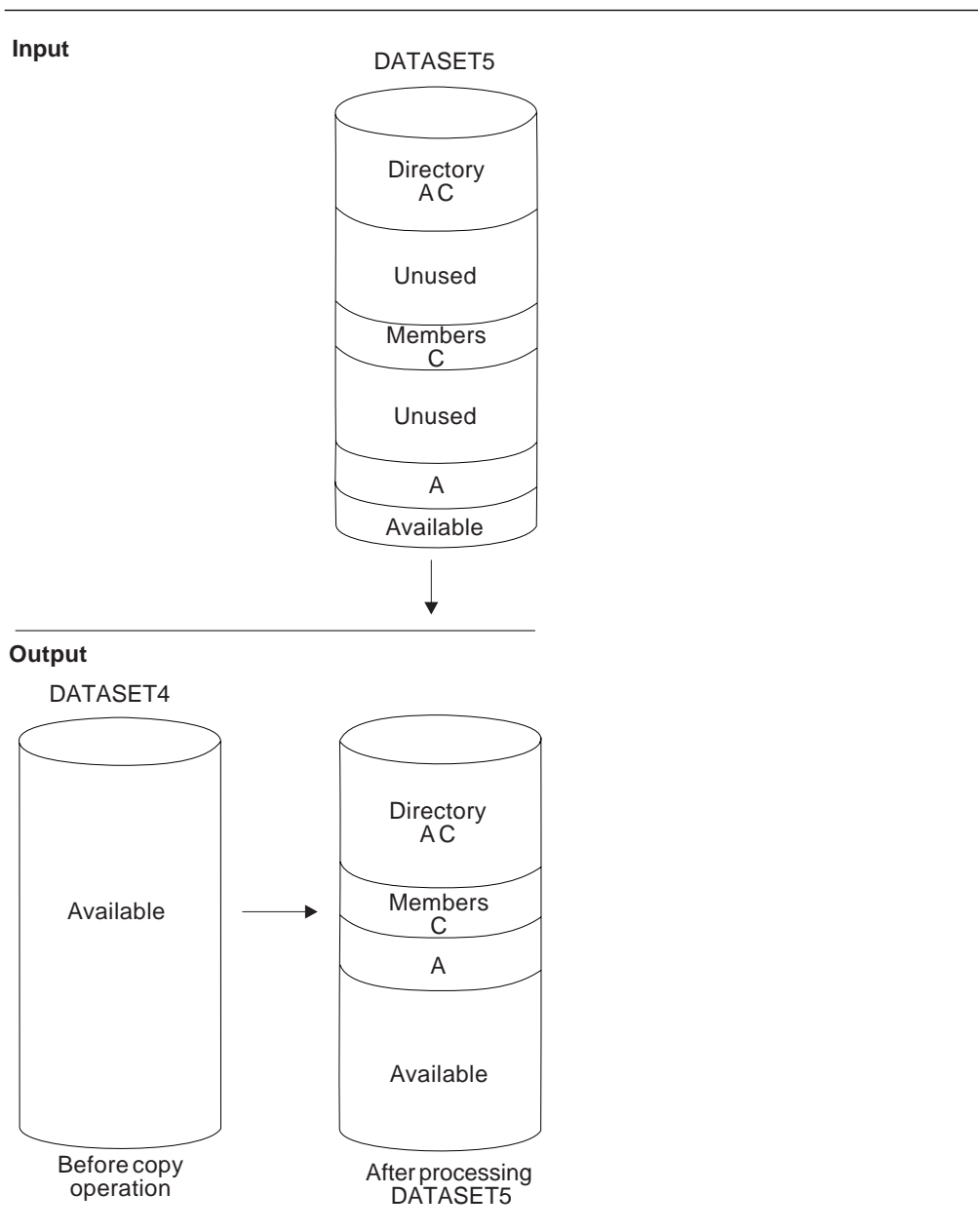
Figure 17. Copying a Partitioned Data Set—Full Copy
