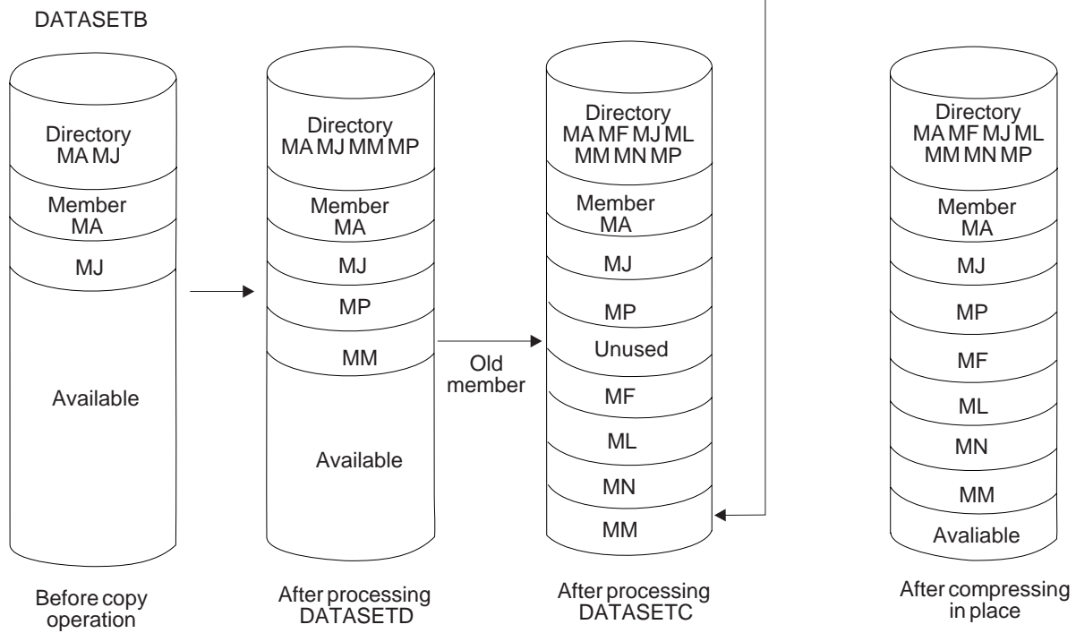
Figure 22 (Part 2 of 3). Multiple Copy Operations/Copy Steps within a Job Step
