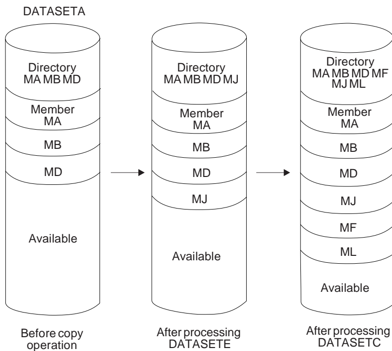
Figure 22 (Part 1 of 3). Multiple Copy Operations/Copy Steps within a Job Step
